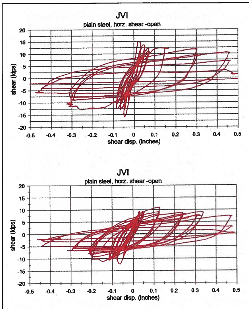
Fig. 3. Shear-to-shear displacement relationships of plain carbon steel connectors under cyclic horizontal shear with joint opening. Courtesy: JVI Inc., Lincolnwood, Illinois.
