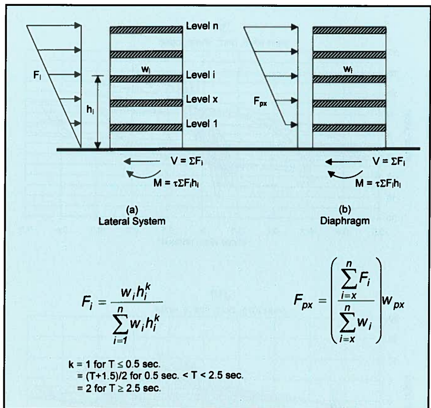
Fig. 2. Equivalent lateral forces for (a) lateral-force-resisting system, (b) diaphragm.
