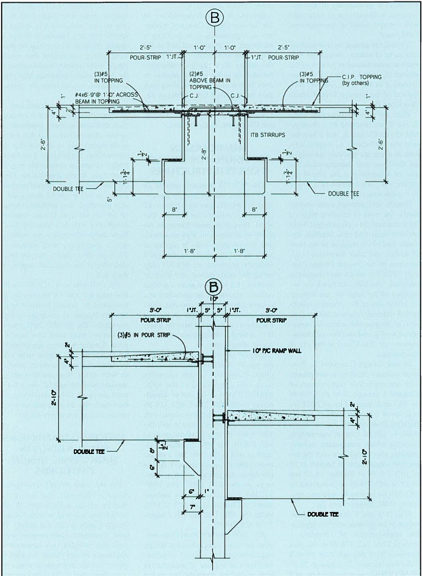
Fig. 1. Cast-in-place pour strips as part of untopped precast diaphragms.
